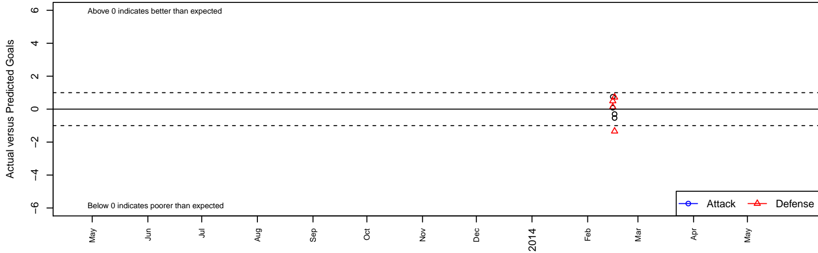
Lake Forest SA G01 Dots are actual minus expected GF (blue circles) and GA (red triangles). Blue line is smoothed change in attack strength. Red is smoothed change in defense strength.
